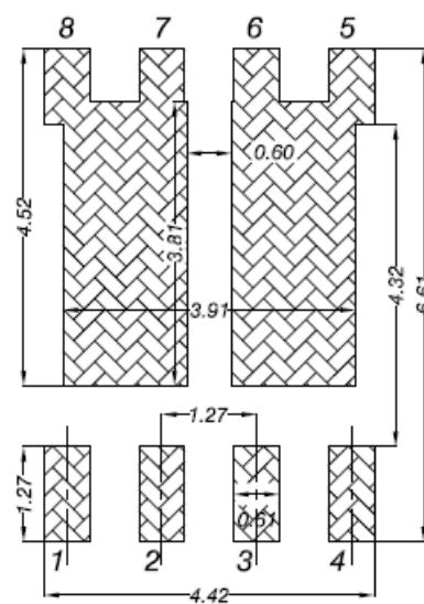
Land Pattern (Only for Reference)
