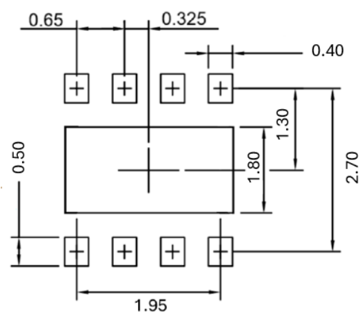
Land Pattern (Only for Reference)
