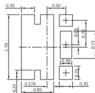
Land Pattern (Only for reference)
