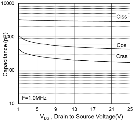
Fig.7 Capacitance
